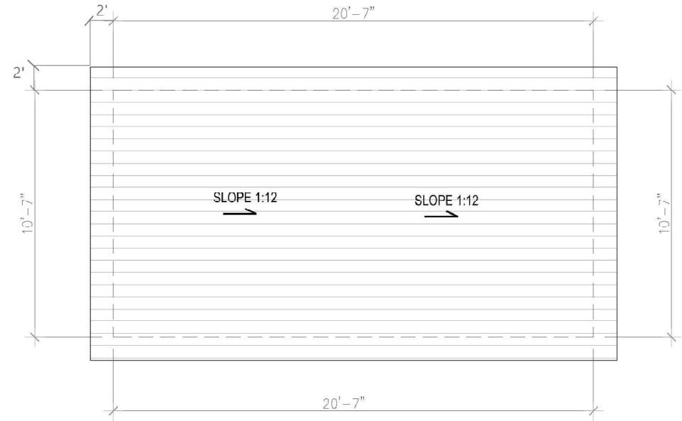
2 ROOF FLOOR PLAN Scale 1"=1/4"
