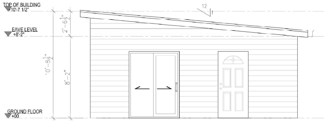
4 FRONT ELEVATION Scale 1"=1/4"
