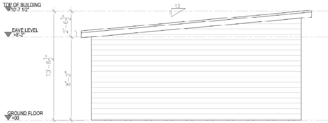
3 BACK ELEVATION Scale 1"=1/4"
