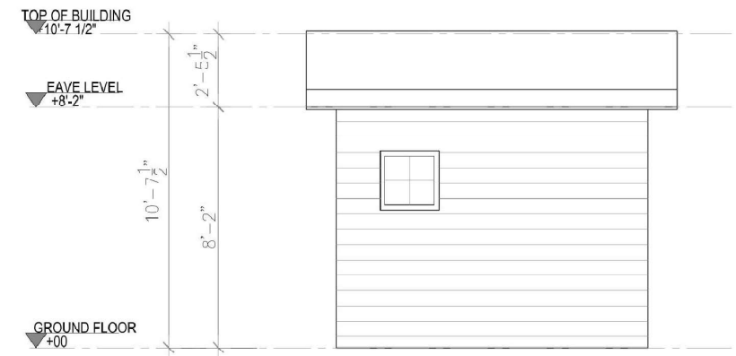
4 LEFT SIDE ELEVATION Scale 1"=1/4"
