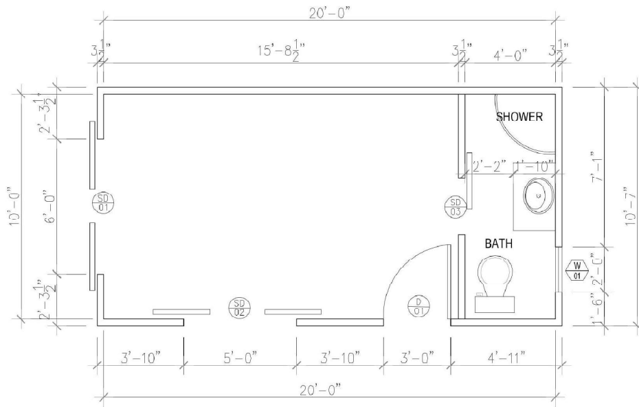
1 GROUND FLOOR PLAN Scale 1"=1/4"
